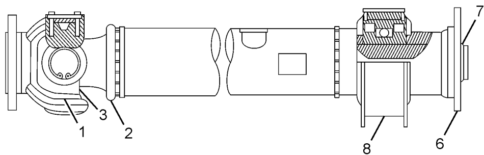
FRONT PROPELLER SHAFT
